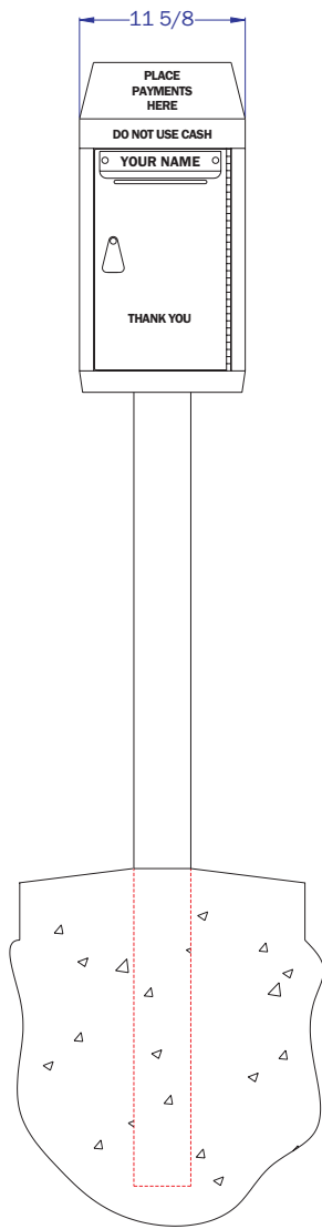
FRONT VIEW
